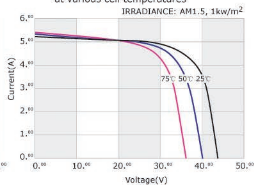
I-V Curves of PV module TSM-175-DC01 at various cell temperatures
