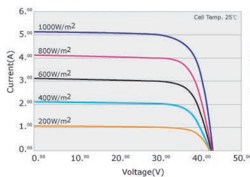
I-V Curves of PV module TSM-175-DC01
