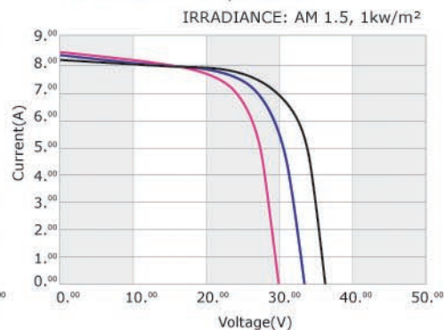
I-V Temperature I-V Curves of TSM-230-DC05 at various cell temperatures
